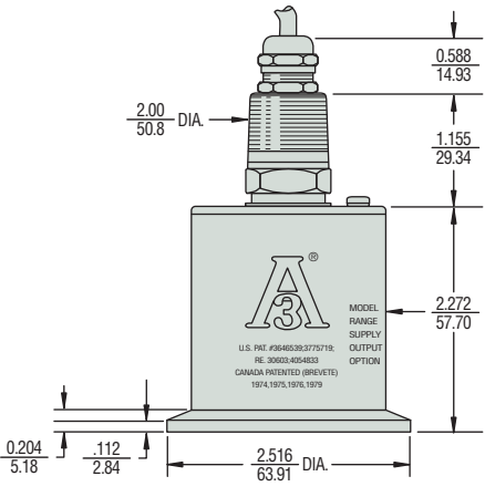
2" Fitting
