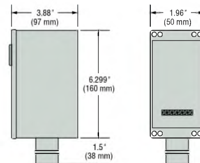
RA-431 shown. TA Series includes an additional 1/2" NPT conduit connection for power.
